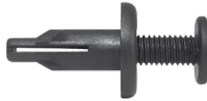
247-495 Std. Pkg. 25 pcs. Head Dia. 18mm, Stem Length: 21mm HONDA Accord 1990-on Push Type Retainer Fits into 8mm Hole #90505-SM4-003 CL Part No: 910-0715, Pieces: 1
